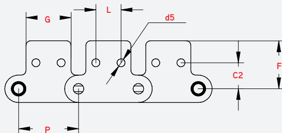
Straight attachment 2 holes 1 side SA-2
