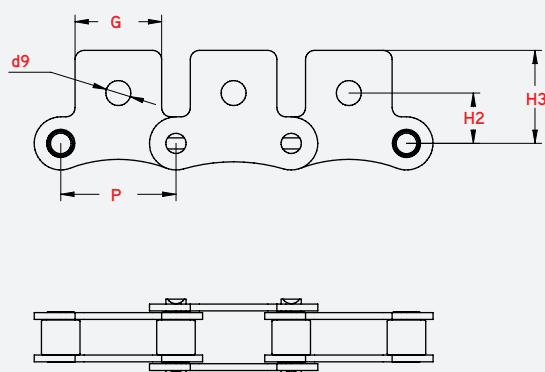
Straight attachment 1 hole 1 side SA-1
