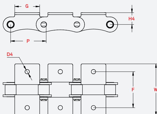
Attachment 90° 1 hole 1 side A-1 Attachment 90° 1 hole 2 sides K-1
